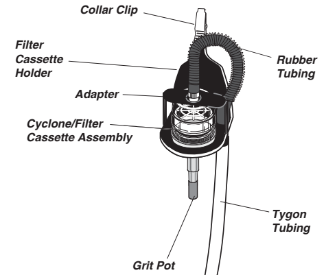
Figure 3 Cyclone with filter cassette in holder
