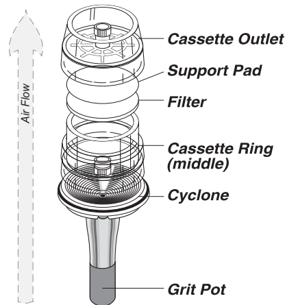
Figure 1 Exploded view of the cyclone/filter cassette assembly
