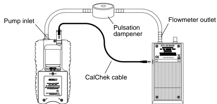
Figure 7. CalChek Full Calibration Train (Leland Legacy Pump)
