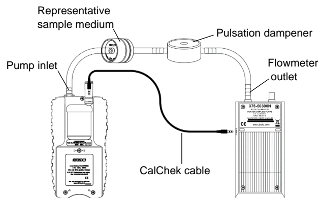
Figure 5. CalChek Single Calibration Train (Leland Legacy Pump)
