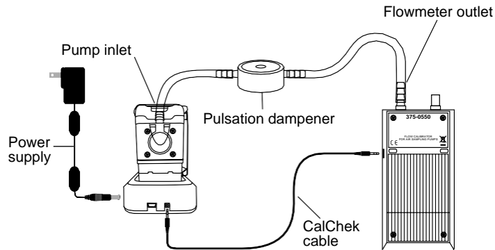
Figure 6. CalChek Full Calibration Train (AirChek TOUCH Pump)
