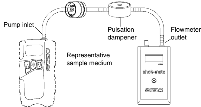
Figure 3. High Flow Calibration Train
